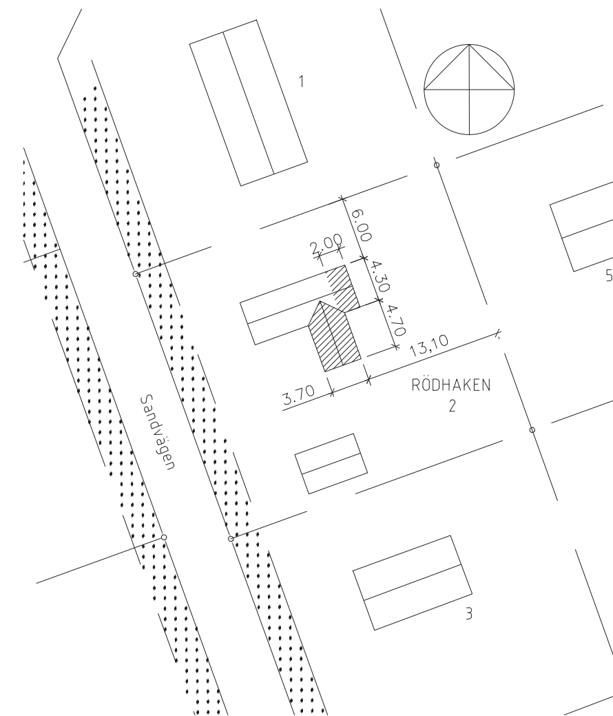
SITUATIONSPLAN SKALA 1:500
